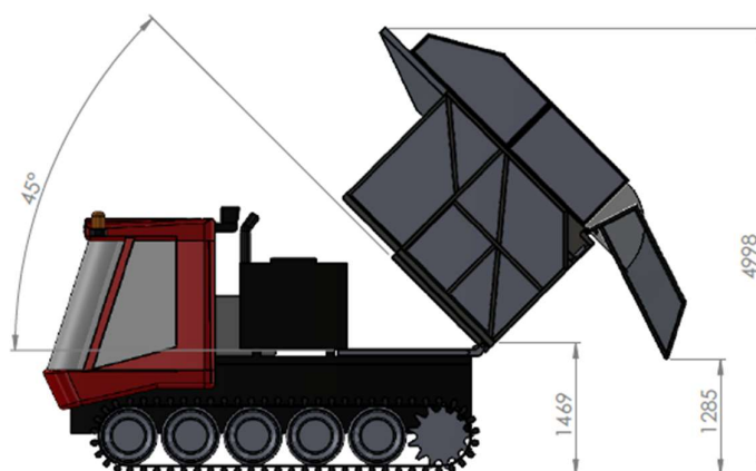
Unloading dimensions
