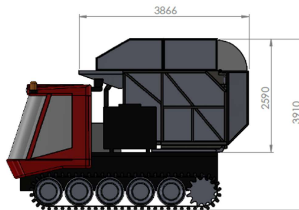
Working dimensions
